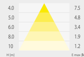
Suprema LED SO 350-P
